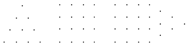
Triangular, square and pentagonal number of order 4
